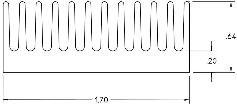
EXTRUSION PROFILE
