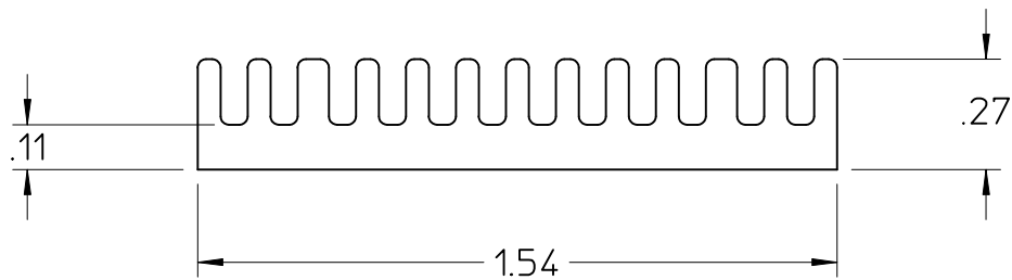
EXTRUSION PROFILE
